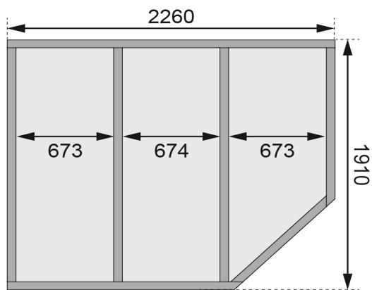
Fundamentplan
