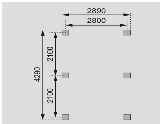
Fundamentplan Pfosten (in mm)
