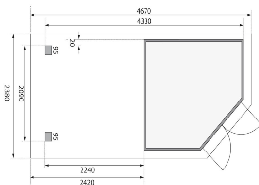
Fundamentplan (in mm)
