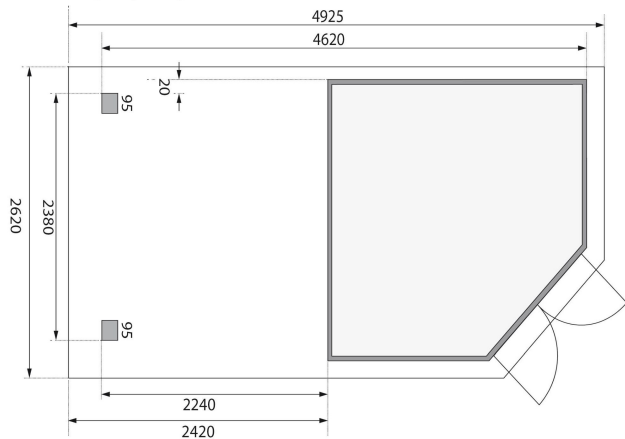
Fundamentplan (in mm)
