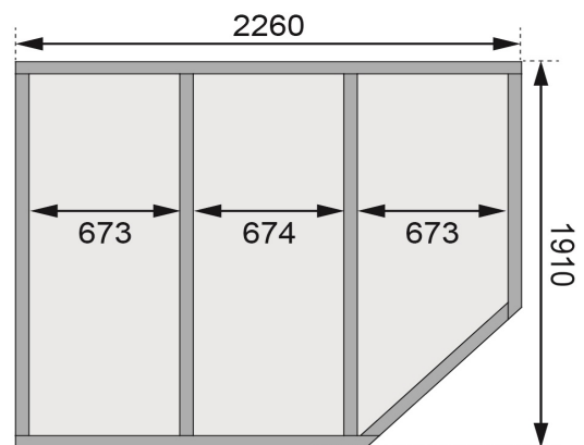
Fundamentplan
