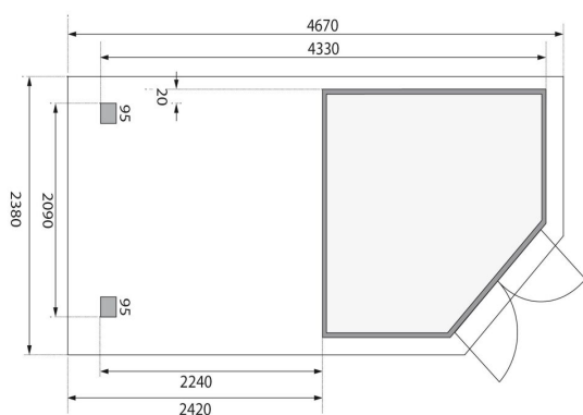
Fundamentplan (in mm)
