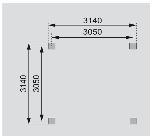
Fundamentplan Pfosten (in mm)
