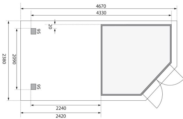
Fundamentplan (in mm)
