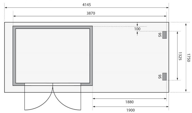
Fundamentplan (in mm)
