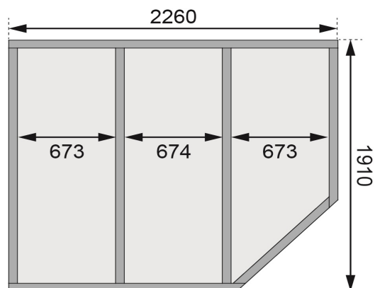
Fundamentplan
